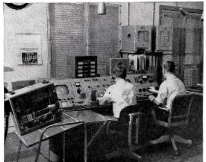
Two engineers control WNAO's entire program schedule—slides, film, studio and network—with Federal Transm Control Console and Poly-Efex Scanner providing complete transmitter supervisory control and audio/video switch. Scanner includes 2 slide sources, four-channel video switch and "special effects" section.
